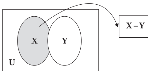
Figure 17.6. Venn Diagram for X - Y
